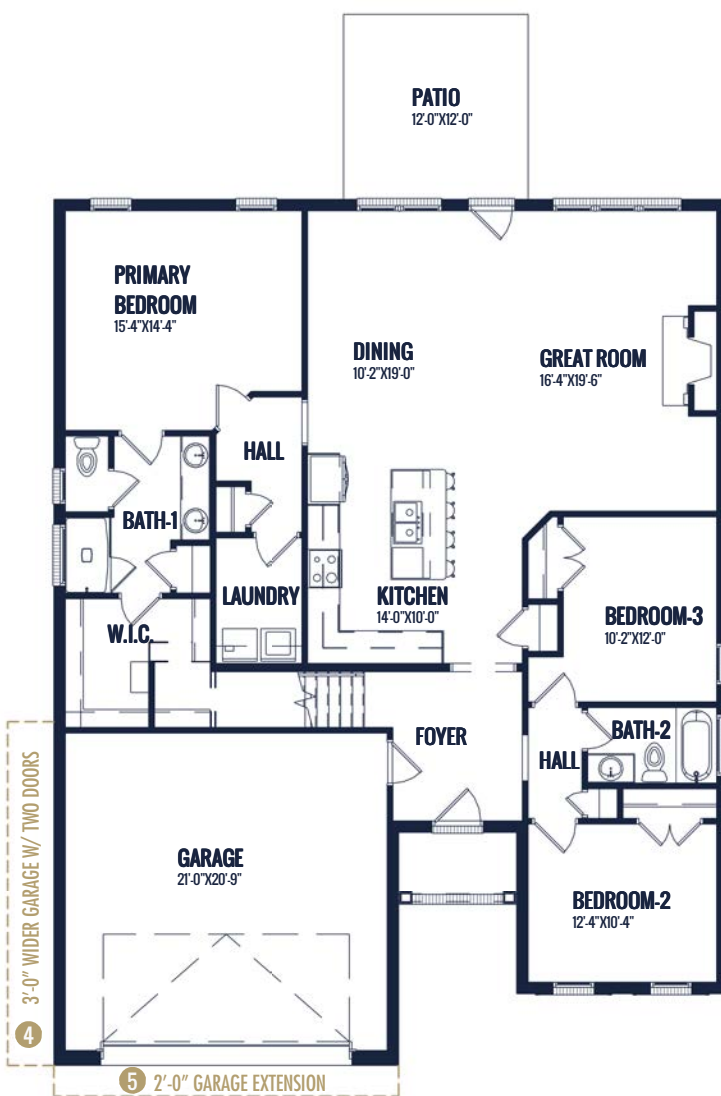
MAIN LEVEL
